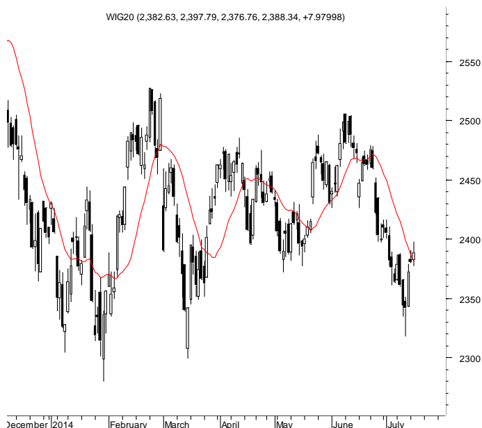
WIG20 (2,382.63, 2,397.79, 2,376.76, 2,388.34, +7.97998)
