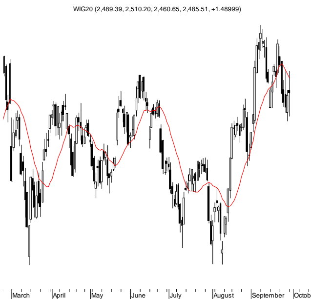
WIG20 (2,489.39, 2,510.20, 2,460.65, 2,485.51, +1.48999)
